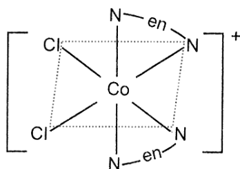
Cis-isomer
