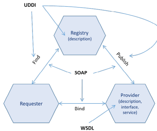
Figure 1-8 Web Service Architecture
