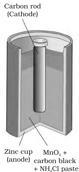
Fig. 3.8: A commercial dry cell consists of a graphite (carbon) cathode in a zinc container; the latter acts as the anode.
