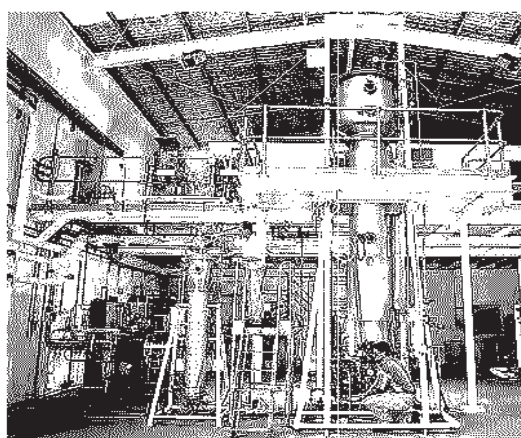
Figure 10.5 Fermentation Plant
