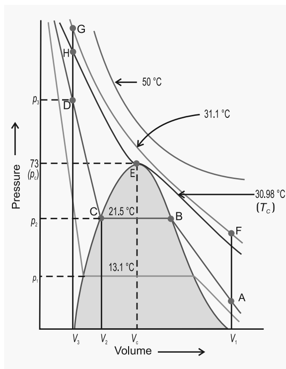
Fig. 5.11 Isotherms of carbon dioxide at various temperatures
