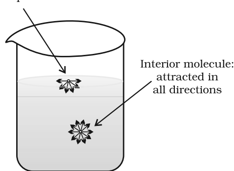
Fig. 5.13 Forces acting on a molecule on liquid surface and on a molecule inside the liquid
